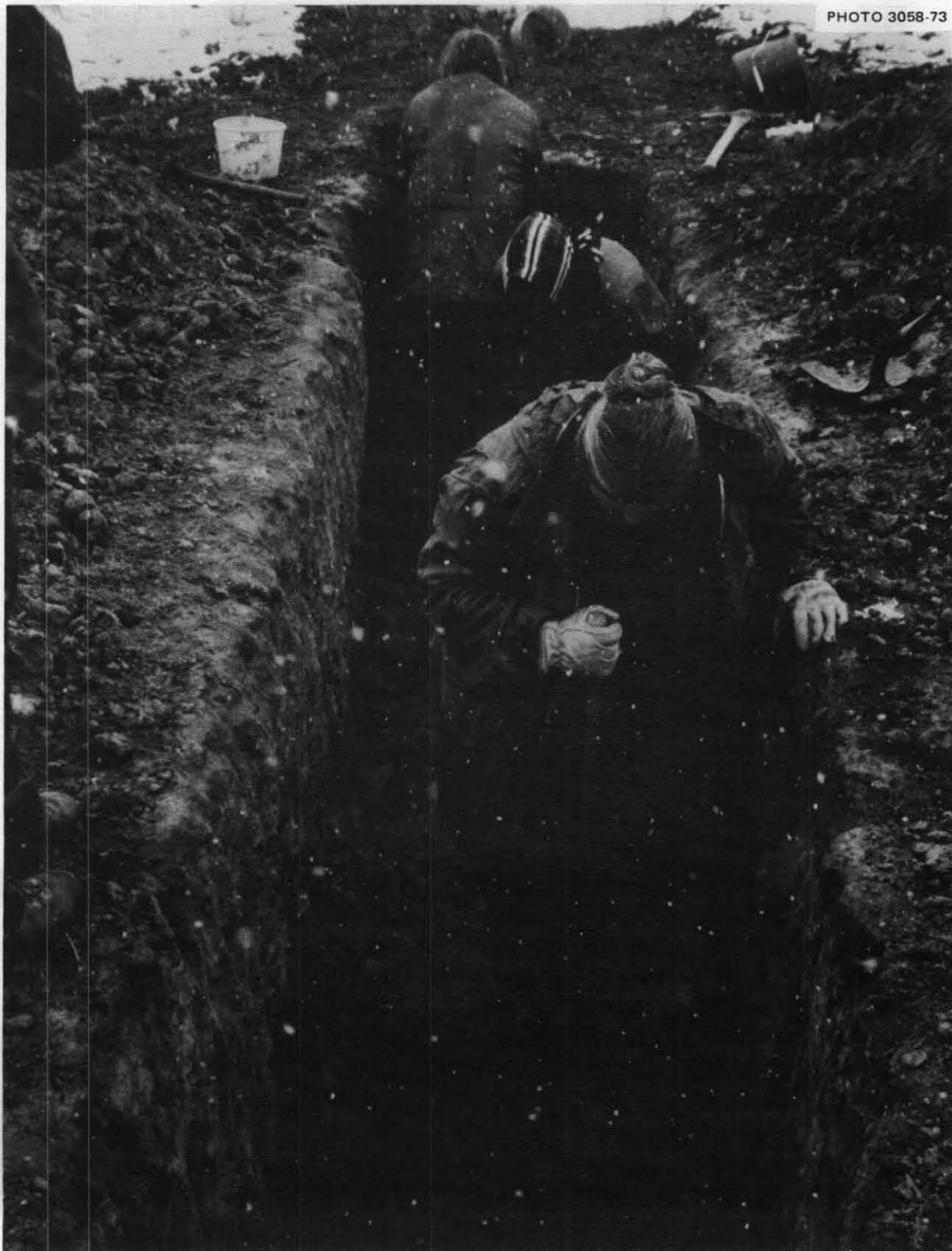
Fig. 2.7. At 8 AM on the second day, when the trench was about 3 ft deep, this family had the good fortune to get below the dry, hard clay-loam and into a slightly sandy clay-loam. The mother could dig this very stable but not-so-hard earth by standing on the shovel and slicing and prying off rows of chunks from the edge of a 6-in.-high earth step.
